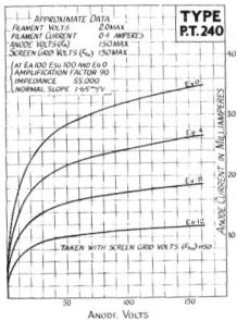
Characteristic Curves of Average PT 240 Valve.
